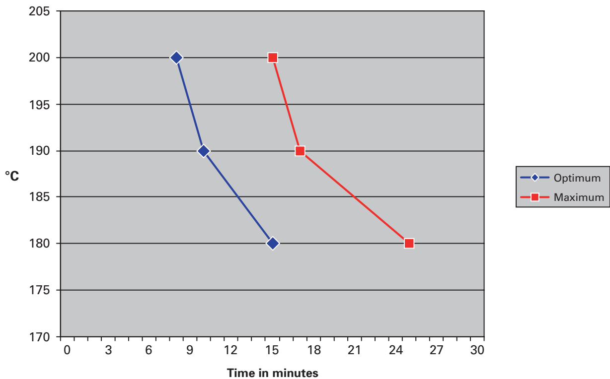
Curing Schedule Alesta AP AE Semi-Gloss 70GU
