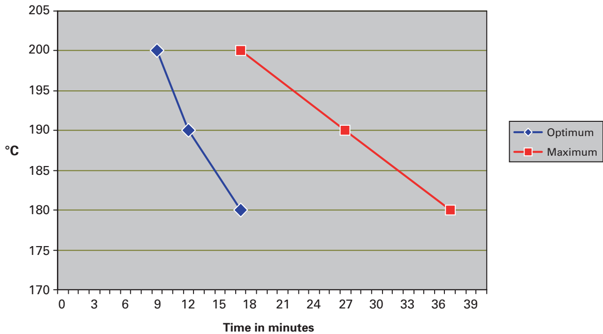
Curing Schedule Alesta AP AE Matt 30GU
