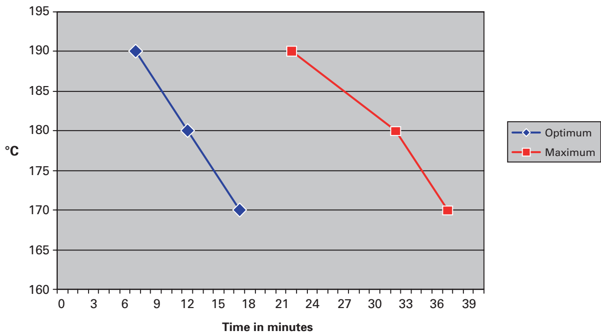
Curing Schedule Alesta AP AE Gloss 85GU
